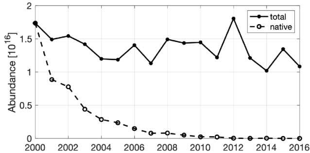
Fig. 8. Number of total and native North Sea C. finmarchicus individuals on 1 January of the period 2000–2016. Native population is defined as the individuals that are found in the North Sea on 1 January of 2000 and their offsprings.
